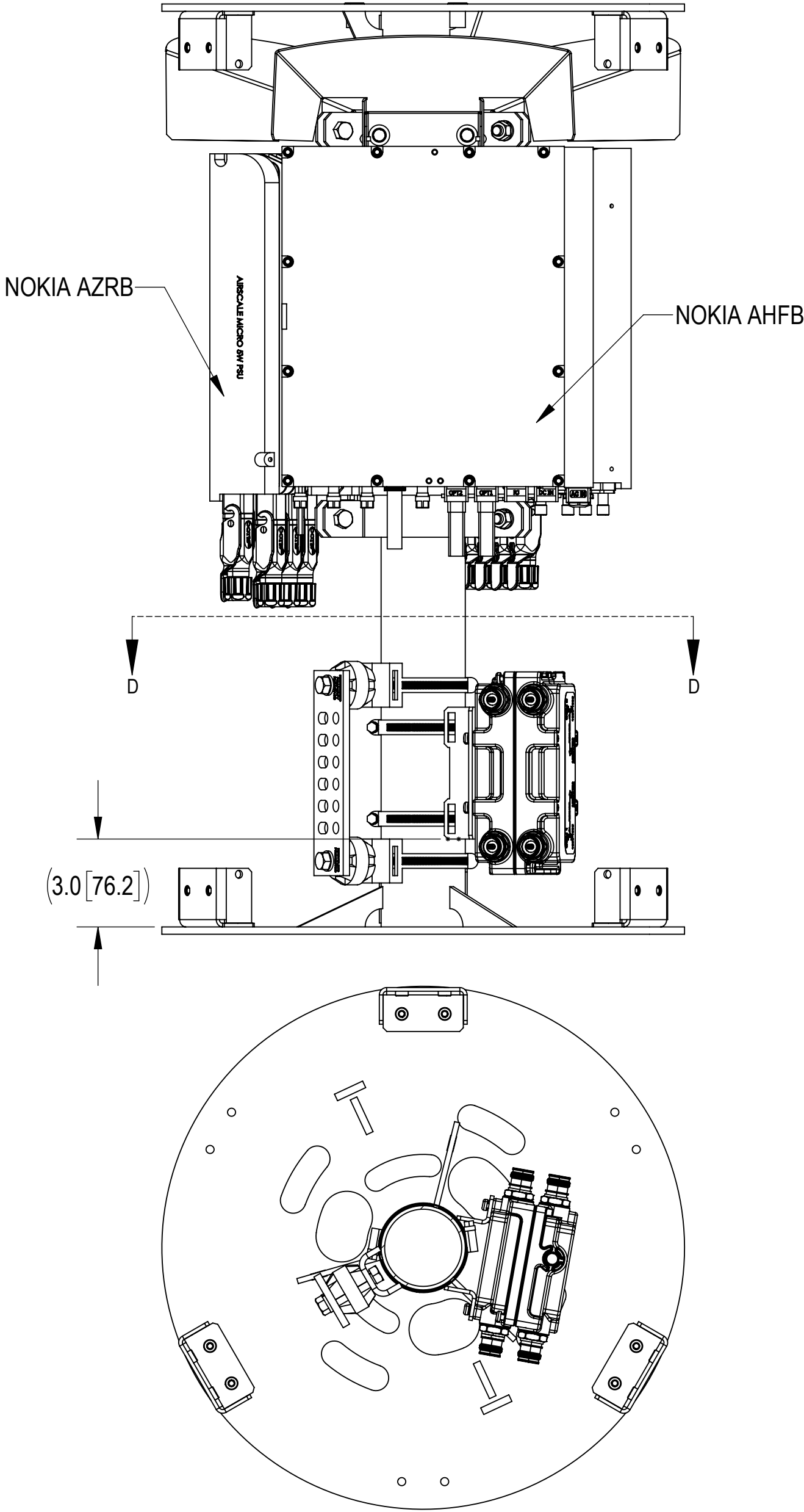
DIPLEXER INSTALLATION OPTION WITH 3 RADIO
